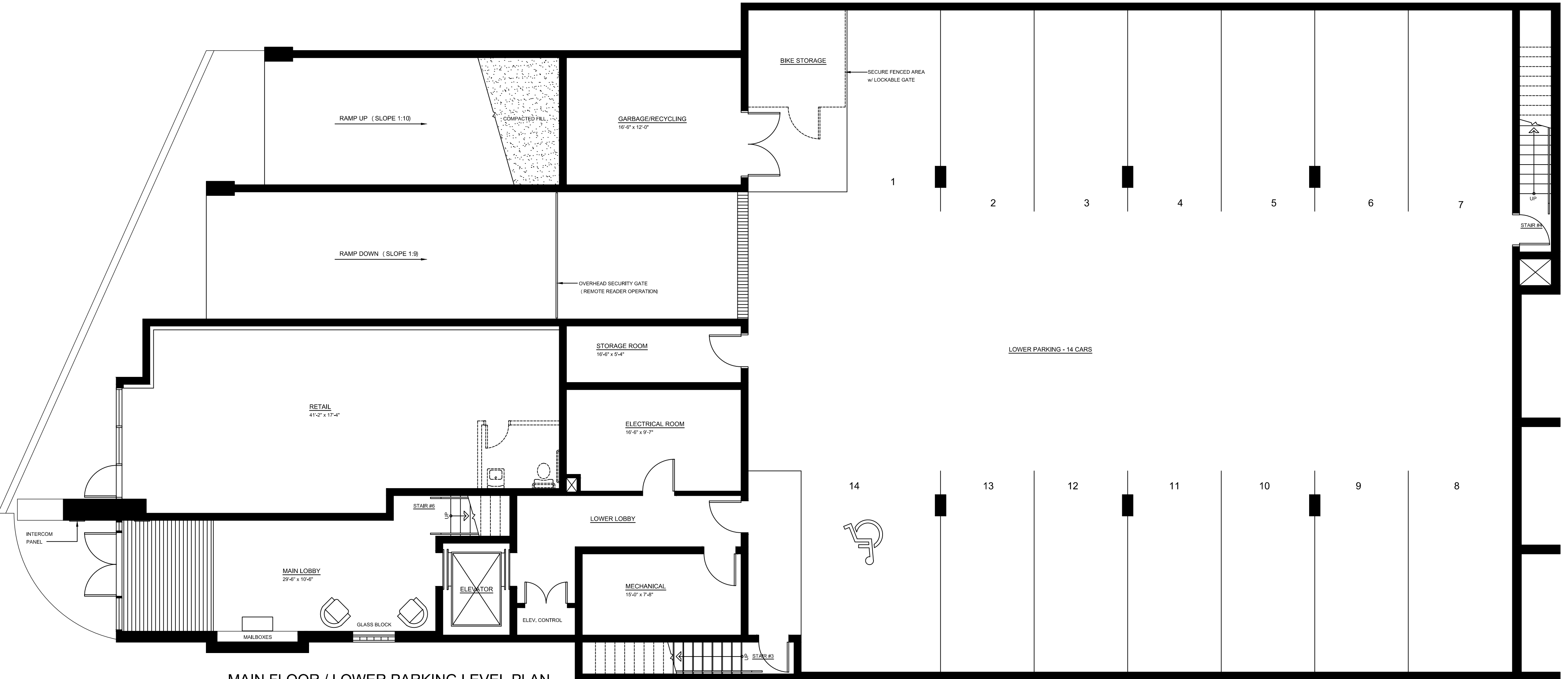
MAIN FLOOR / LOWER PARKING LEVEL PLAN
